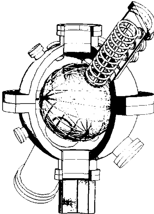
Figure 3.3. Illustration of the IEC Jet Thruster Experiment Showing Central Grid and Two Jet Grids, Opposite to Each Other With On-Off Action
