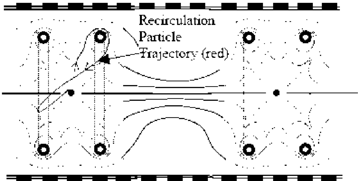
Figure 5.8. Diagram of Belt-Cusp Fields and Particle Recirculation
