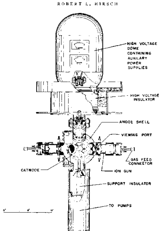
Figure 2.1. The "Historic" Early IEC Ion Injection Experiment of R. Hirsch Working With Philo Farnsworth
