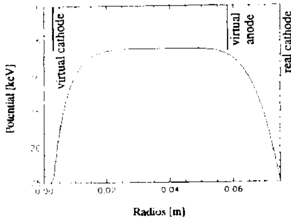
Figure 4.7. The Double Well Potential Calculated With IXL Code for d_{33perp} , i_i=14keV , I_i=55A , I_e=59A
