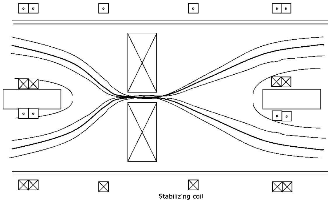
Figure 3.4. Dipole Reactor Propulsion Scheme
