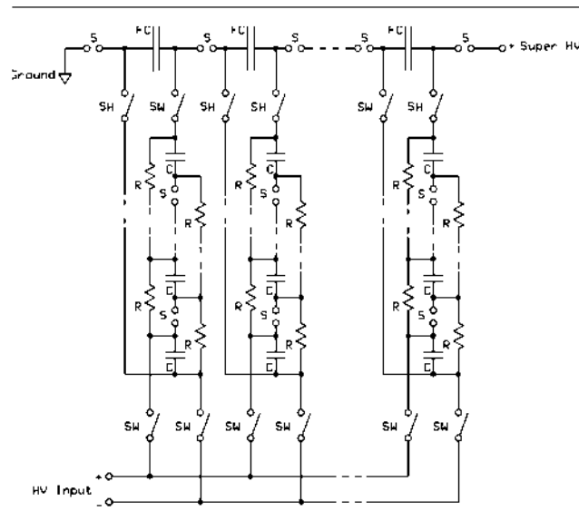
Figure 8. Super Marx Generator. In a Super Marx generator, N Marx generators charge up N fast capacitors FC to the voltage V , which switched into series add up their voltages to the voltage NV .
