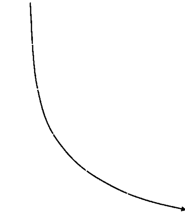
Figure 2. Light-Bending in a Spacetime-Altered Region
