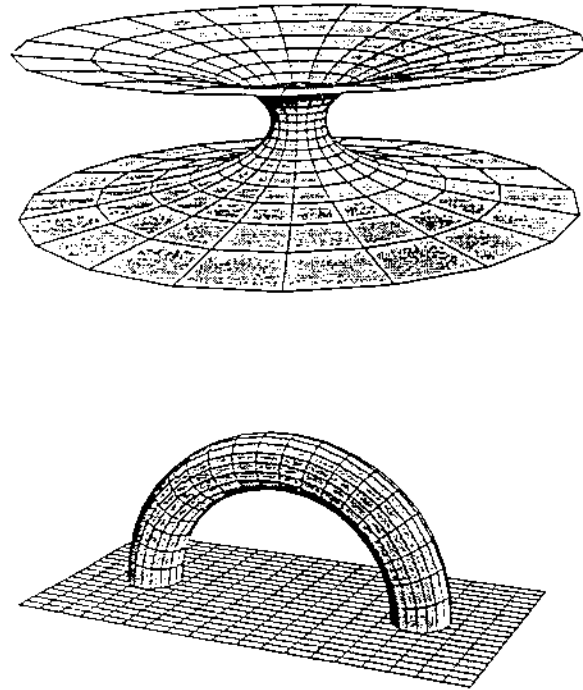
Figure 2. Inter-Universal Wormhole (top) and Intra-Universal Wormhole (bottom).
