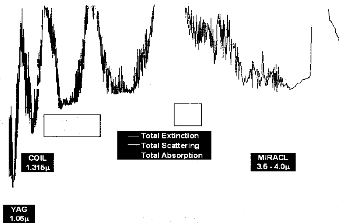
Figure 12. Typical Atmospheric Absorption and Scattering in the Infrared
