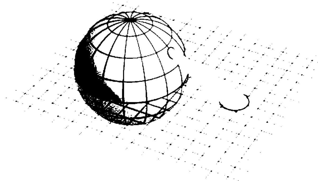
Figure 19. Stereographic Projection
