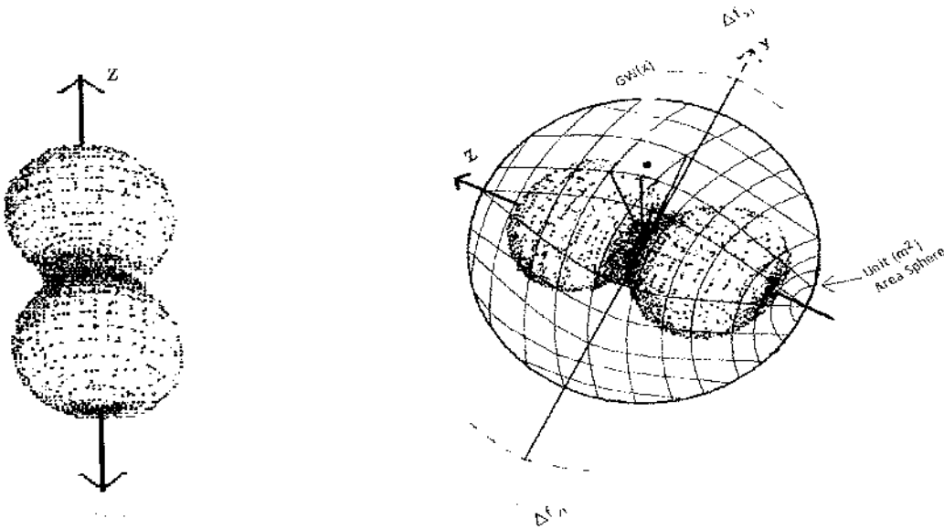
Figure 7. Omni-Directional Nature of the HFGW Radiation Pattern
